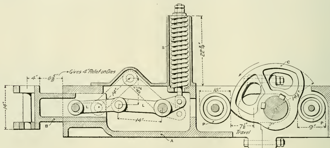
ACME FOUR-INCH UPSETTING MACHINE.
